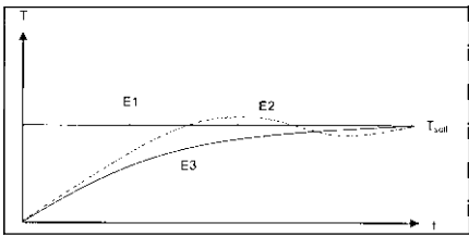
Figure 5: Control characteristics of the individual energy values (schematic)
